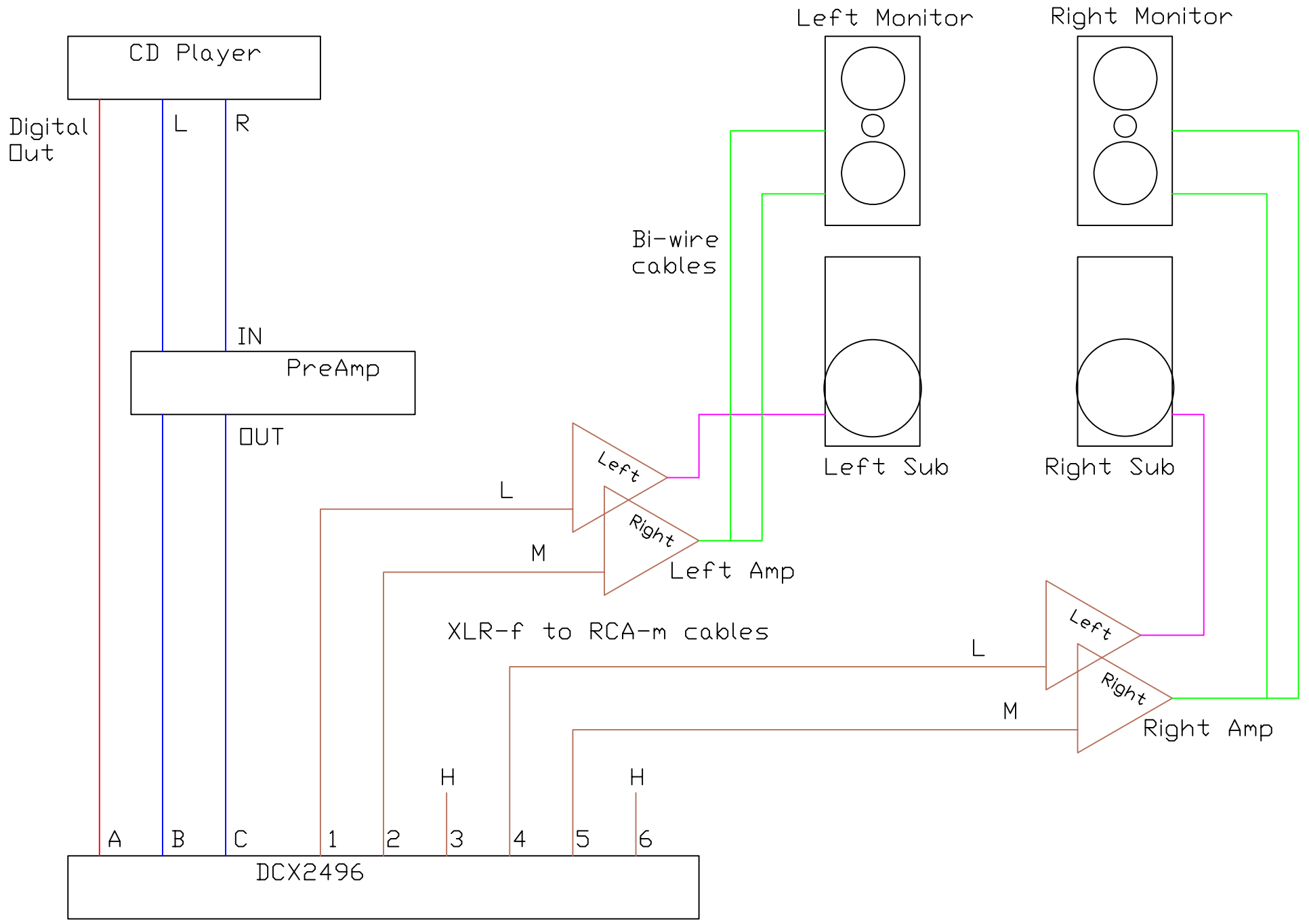
Bi-amp Connection Diagram - BESL
