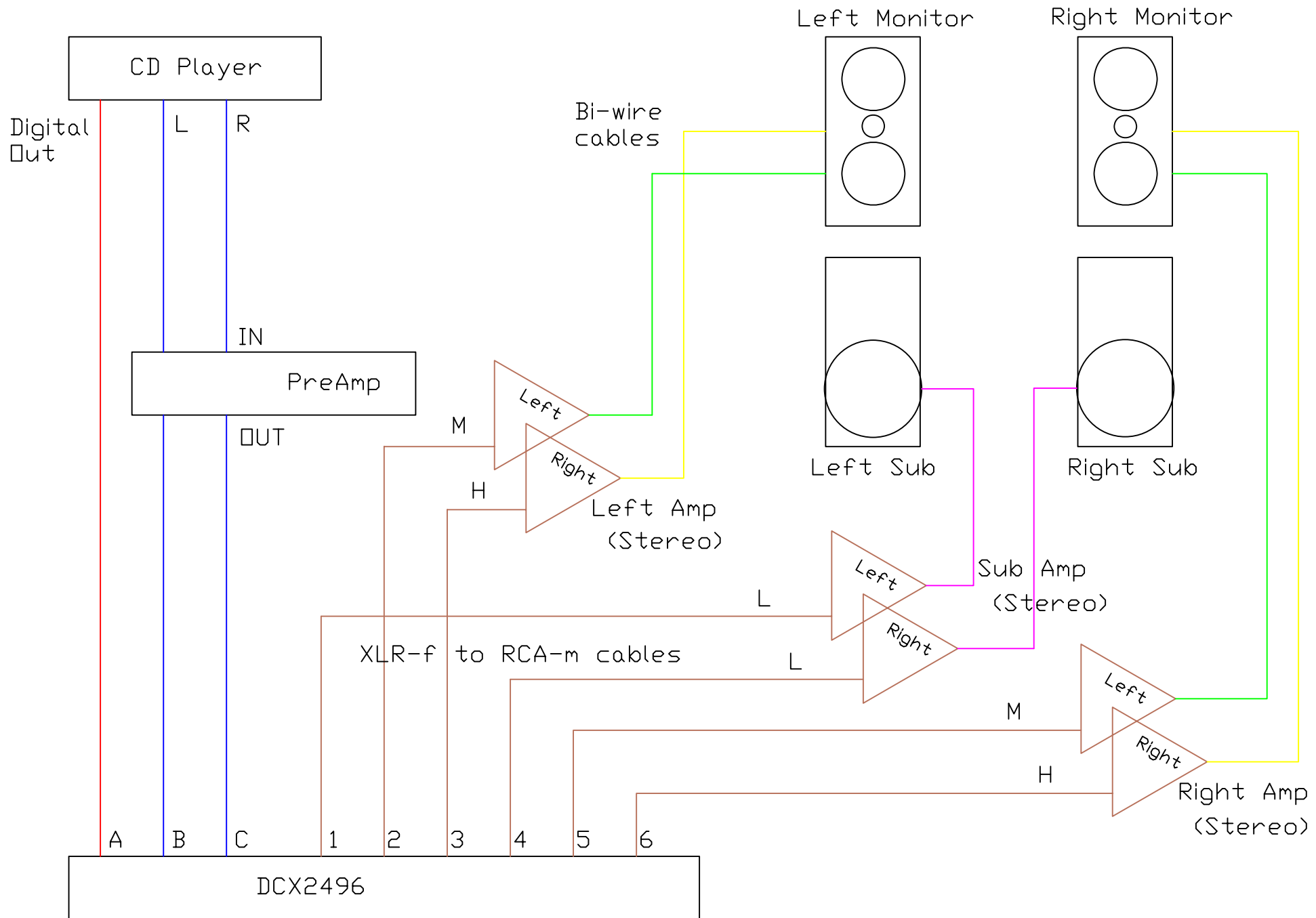
Tri-amp Connection Diagram - BESL
